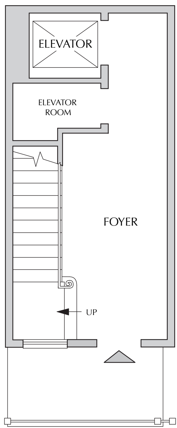
ENTRY LEVEL
